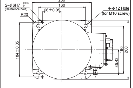
Detailed drawing of base mounting face (Top view)
